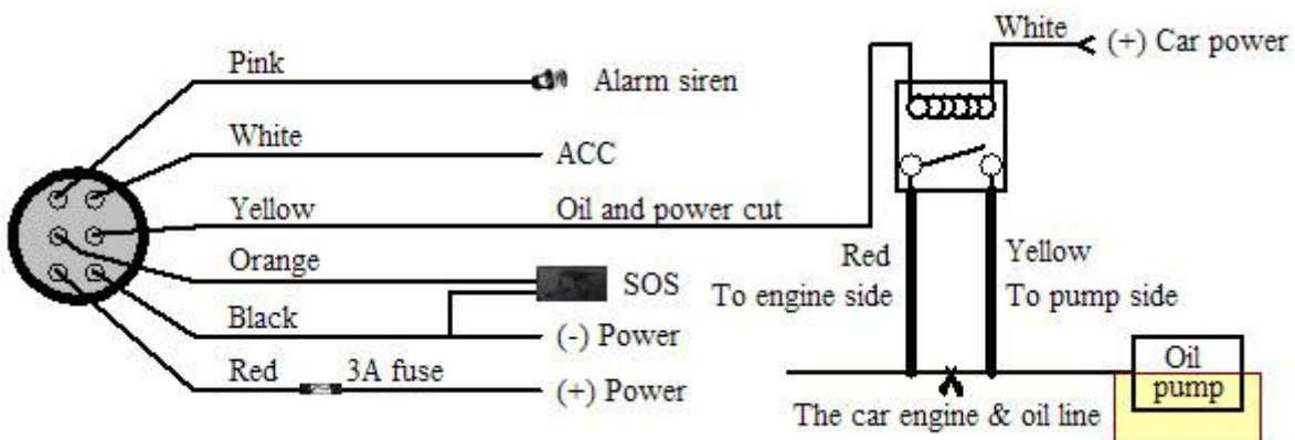
Wiring Diagram
